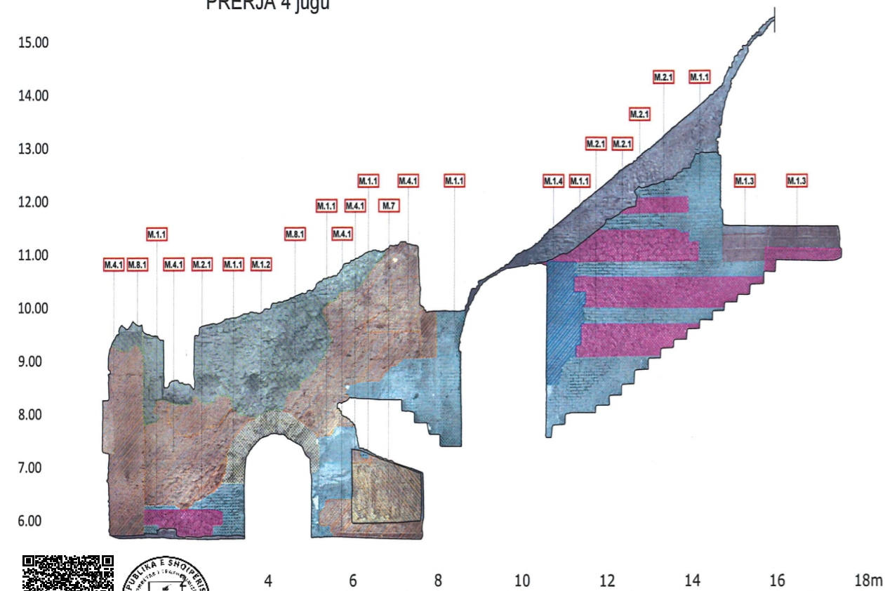
ELEVATION 4 south PRERJA 4 jugu
